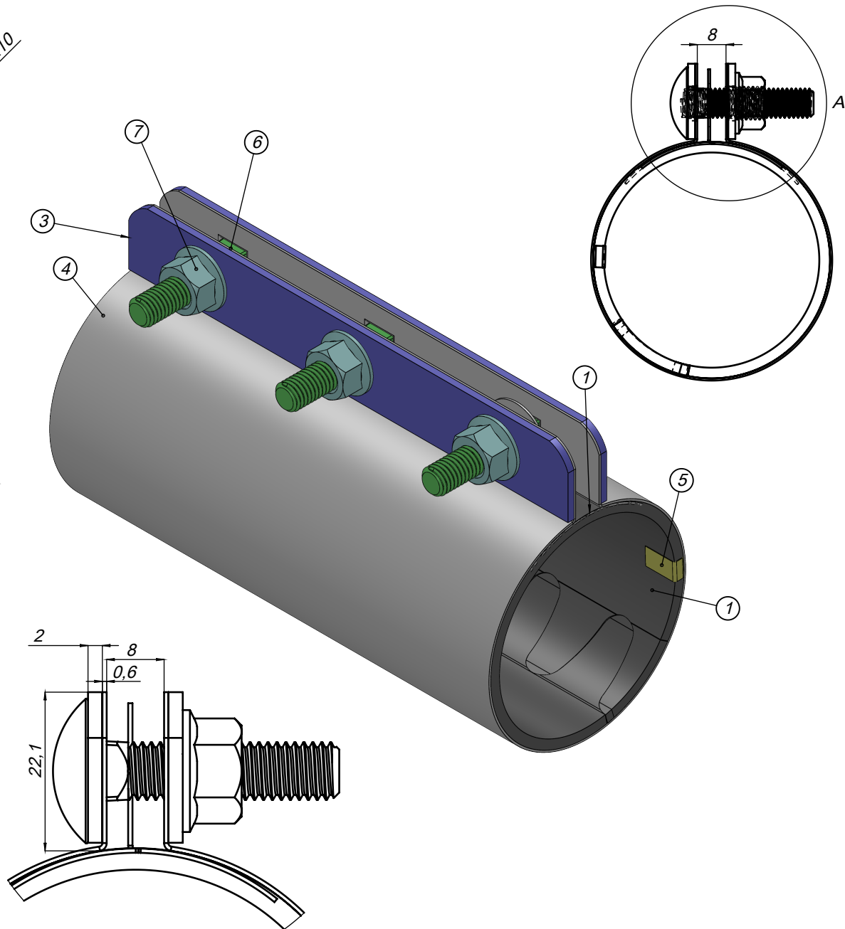
DETAIL A
